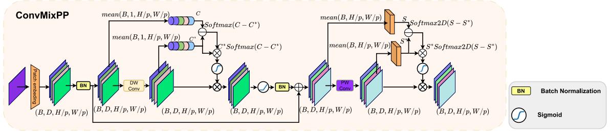
Fig. 2. ConvMixPP block.
